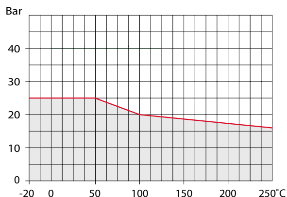
PN 25: Flange × Flange - DN 65 - 200
