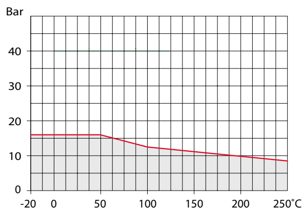
PN 16: Flange × Flange - DN 65 - 200
